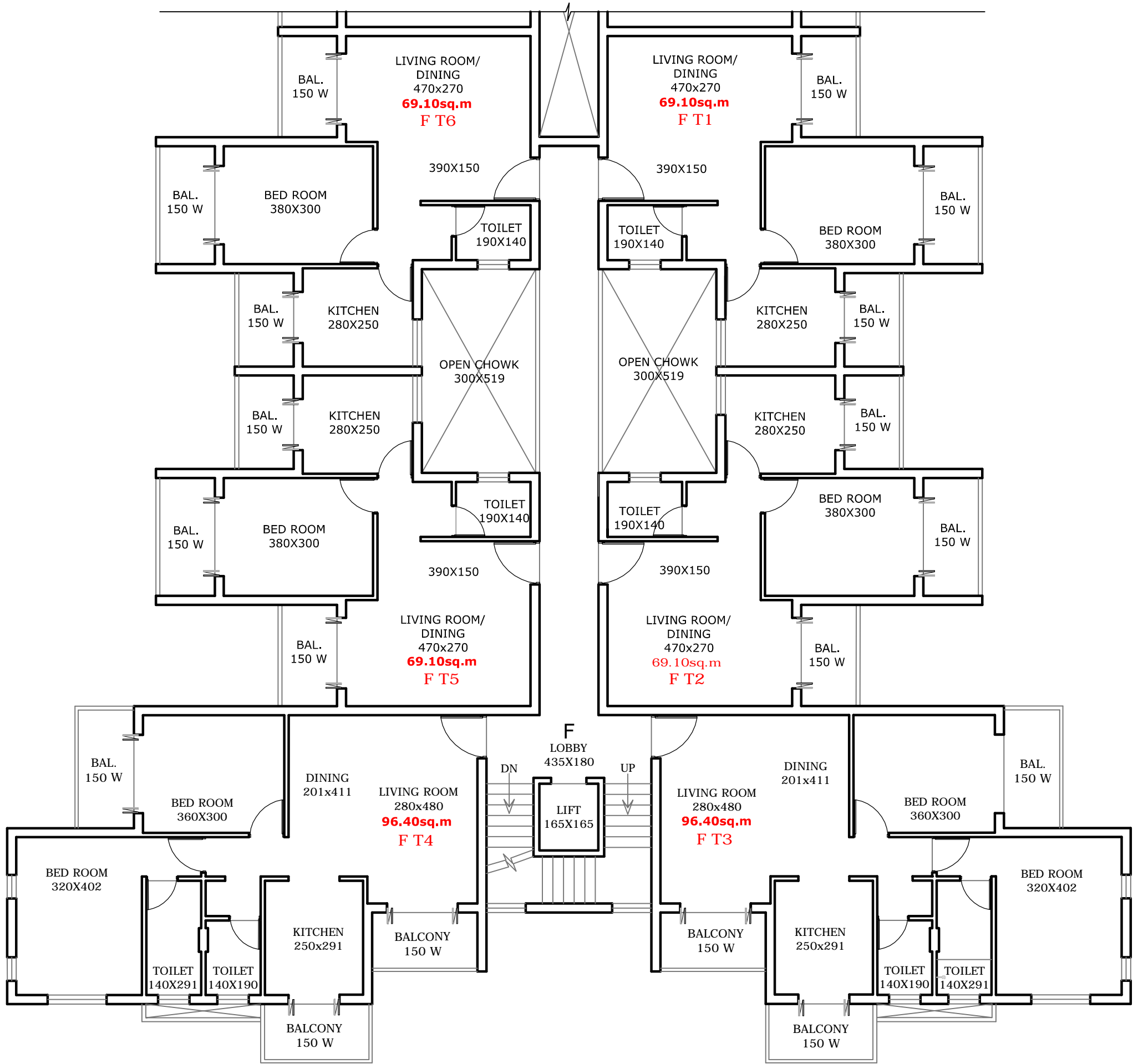
THIRD FLOOR PLAN BUILDING EF - PART F
