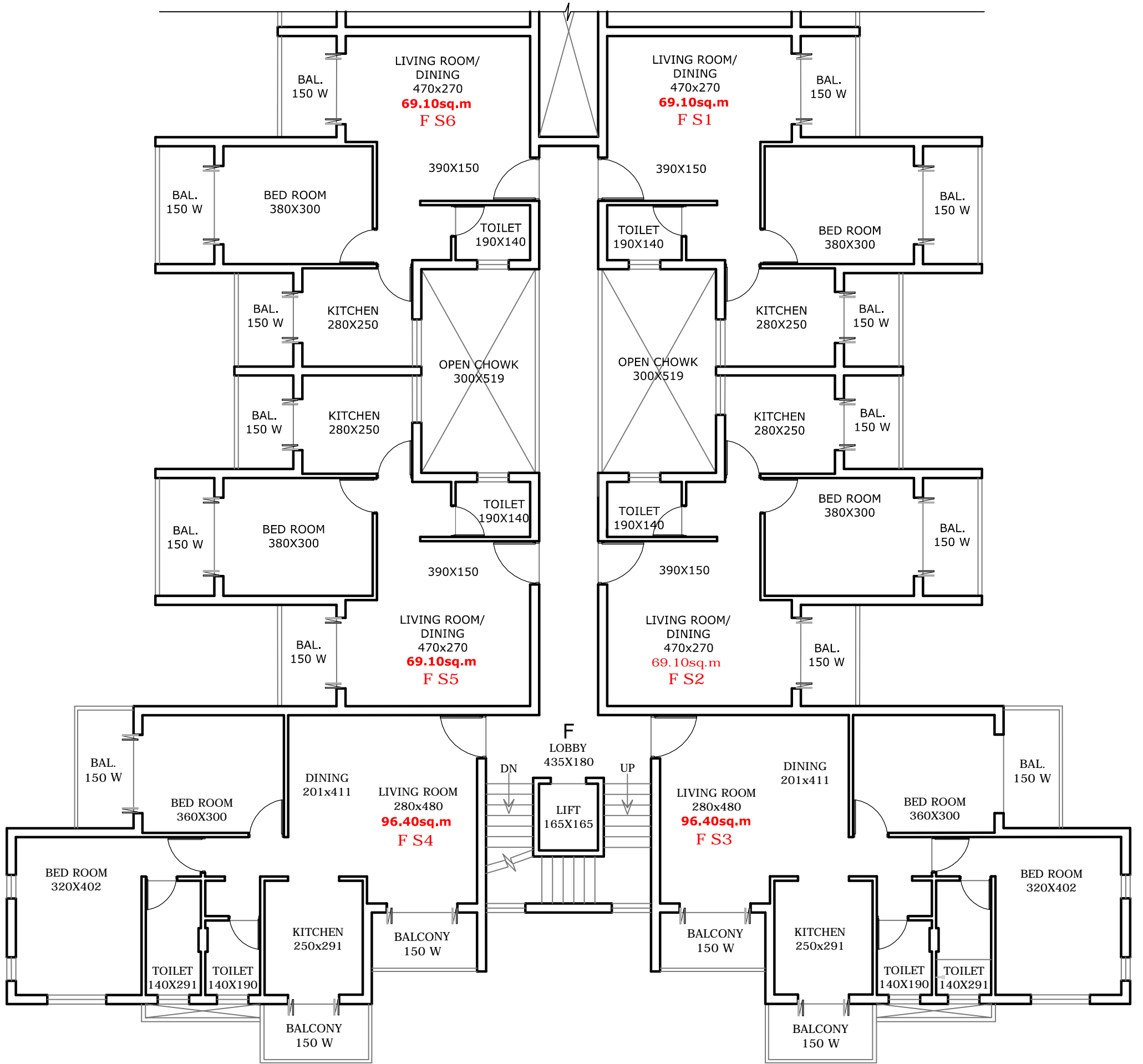
SECOND FLOOR PLAN BUILDING EF - PART F
